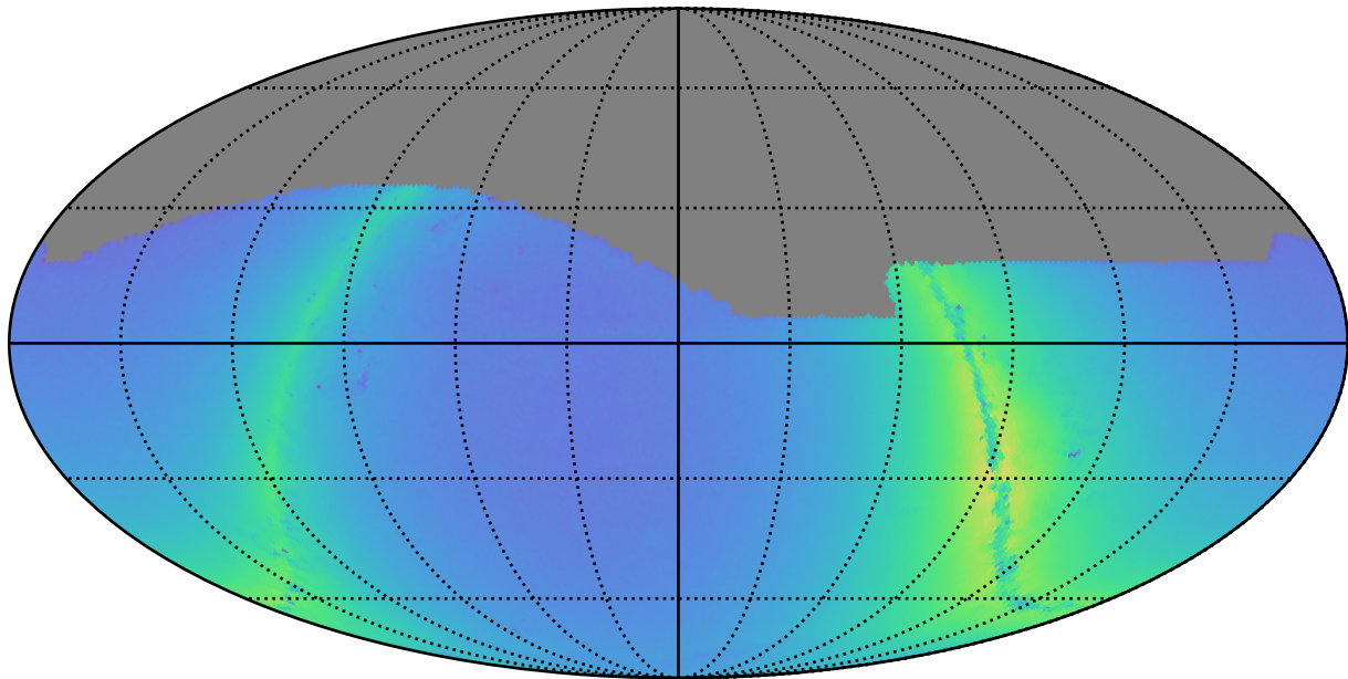
ddf_acor_sf20_lsf40_lsr50_v3.4_10yrs r: Nstars_no_crowding
