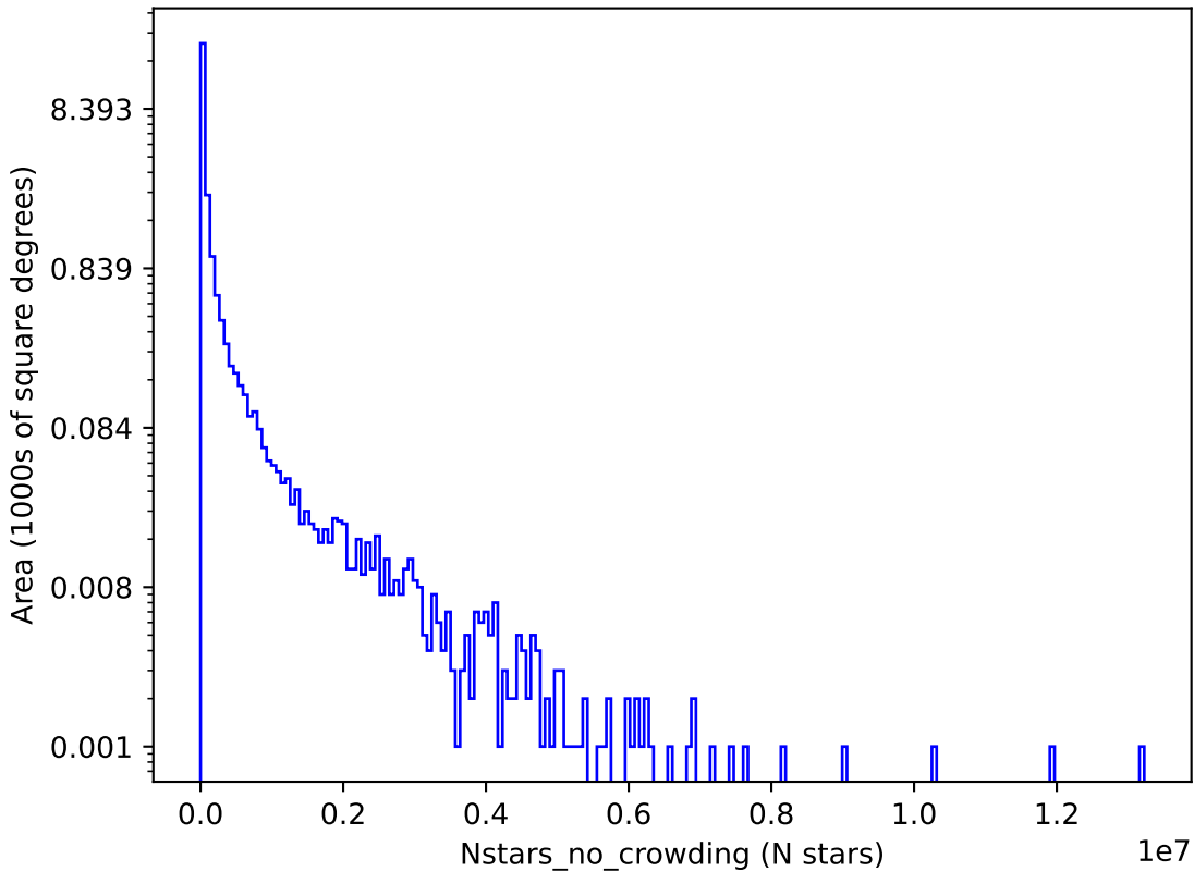
ddf_acor_sf20_lsf40_lsr50_v3.4_10yrs g: Nstars_no_crowding
