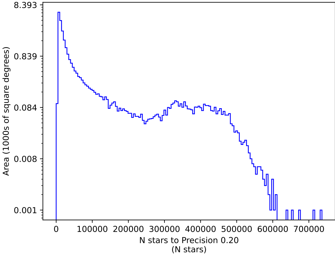
ddf_acor_sf20_lsf40_lsr50_v3.4_10yrs z: N stars to Precision 0.20
