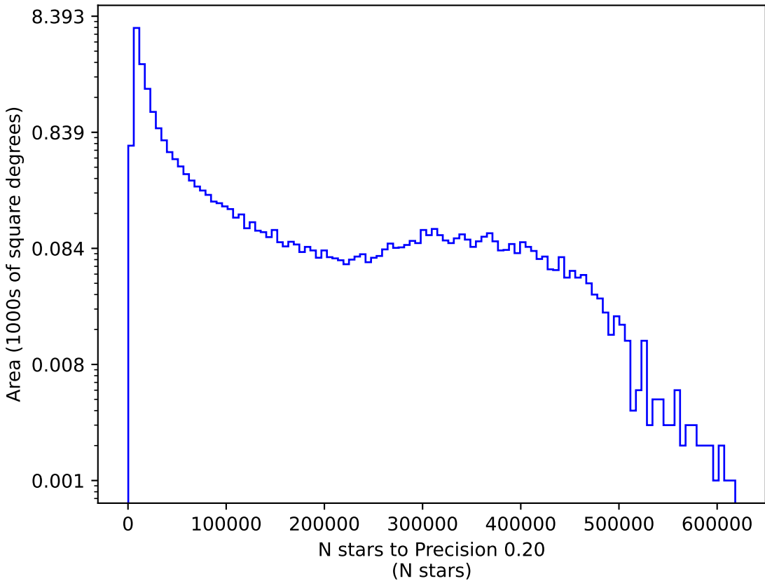
ddf_acor_sf20_lsf40_lsr50_v3.4_10yrs y: N stars to Precision 0.20
