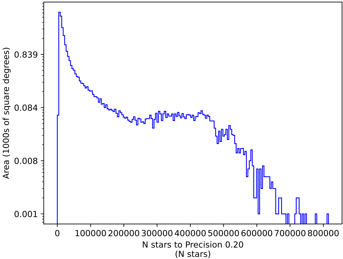
ddf_acor_sf20_lsf40_lsr50_v3.4_10yrs r: N stars to Precision 0.20
