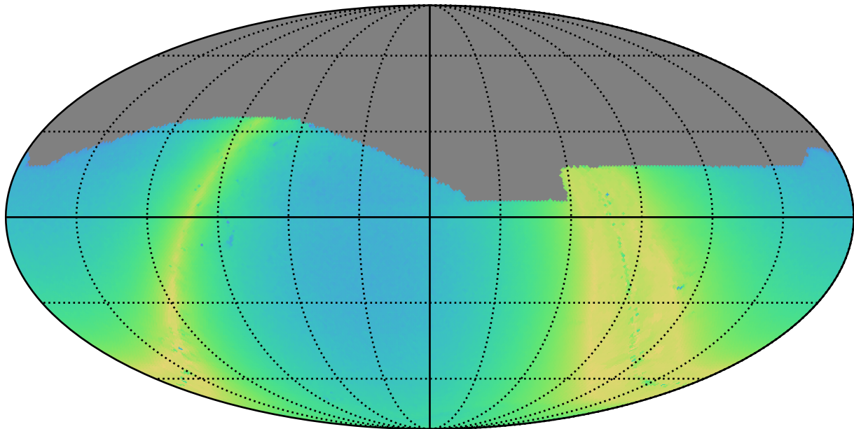
ddf_acor_sf20_lsf40_lsr50_v3.4_10yrs i: N stars to Precision 0.20
