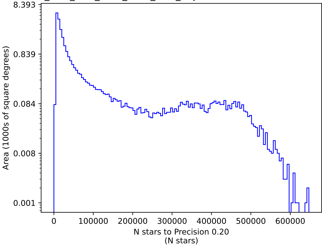
ddf_acor_sf20_lsf40_lsr50_v3.4_10yrs i: N stars to Precision 0.20
