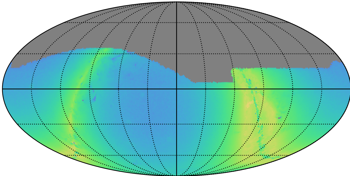
ddf_acor_sf20_lsf40_lsr50_v3.4_10yrs g: N stars to Precision 0.20
