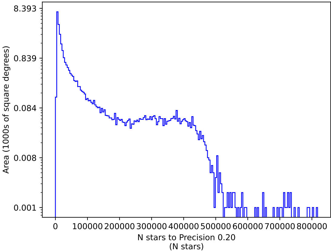
ddf_acor_sf20_lsf40_lsr50_v3.4_10yrs g: N stars to Precision 0.20
