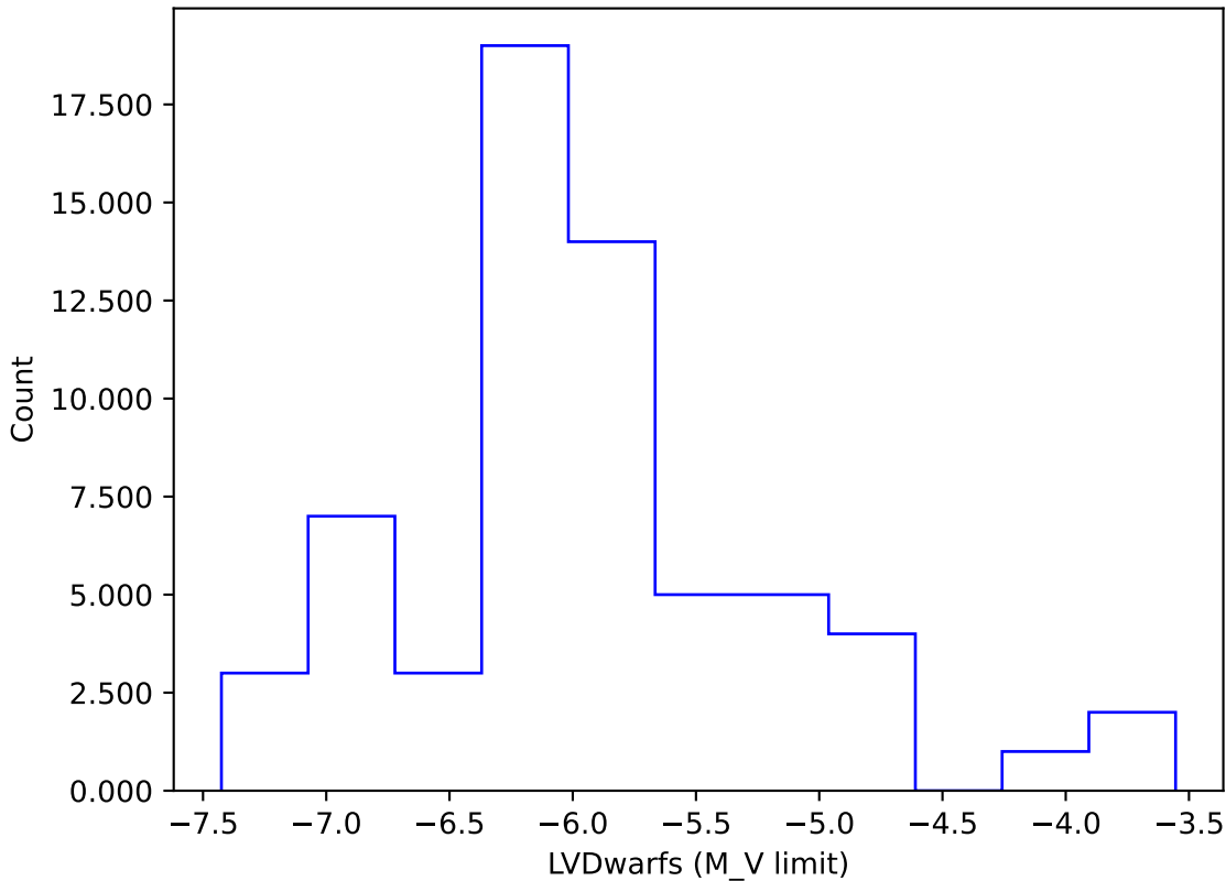
ddf_acor_sf20_lsf40_lsr50_v3.4_10yrs gi: LVDwarfs
