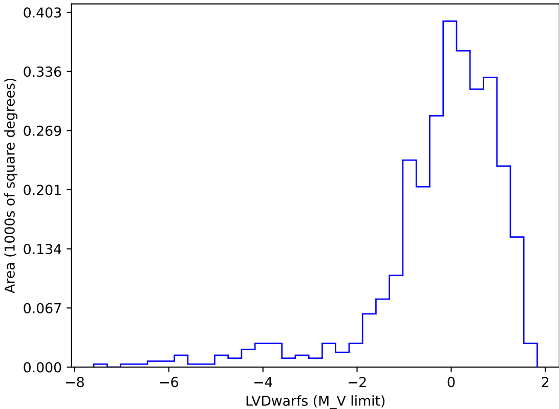
ddf_acor_sf20_lsf40_lsr50_v3.4_10yrs gi SCP: LVDwarfs
