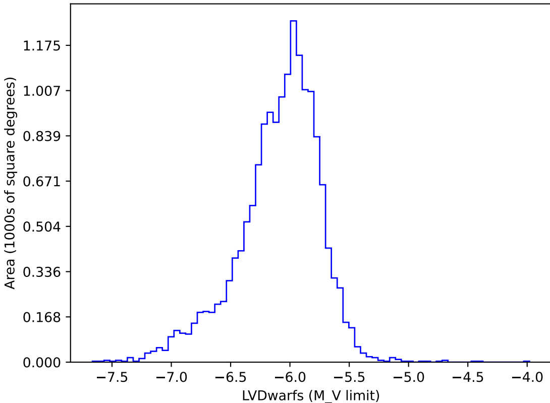
ddf_acor_sf20_lsf40_lsr50_v3.4_10yrs gi: LVDwarfs
