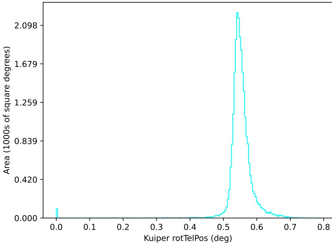
ddf_acor_sf20_ls40_lsr50_v3.4_10yrs u: Kuiper rotTelPos
