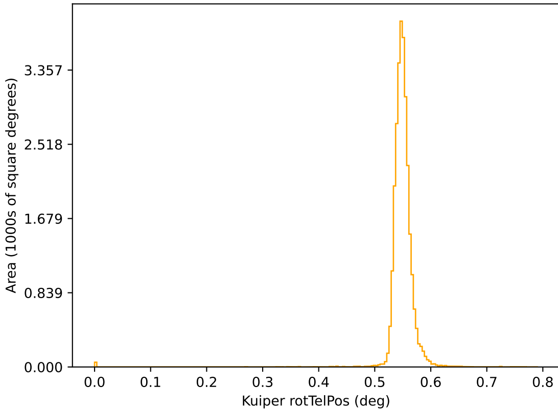
ddf_acor_sf20_lsf40_lsr50_v3.4_10yrs r: Kuiper rotTelPos
