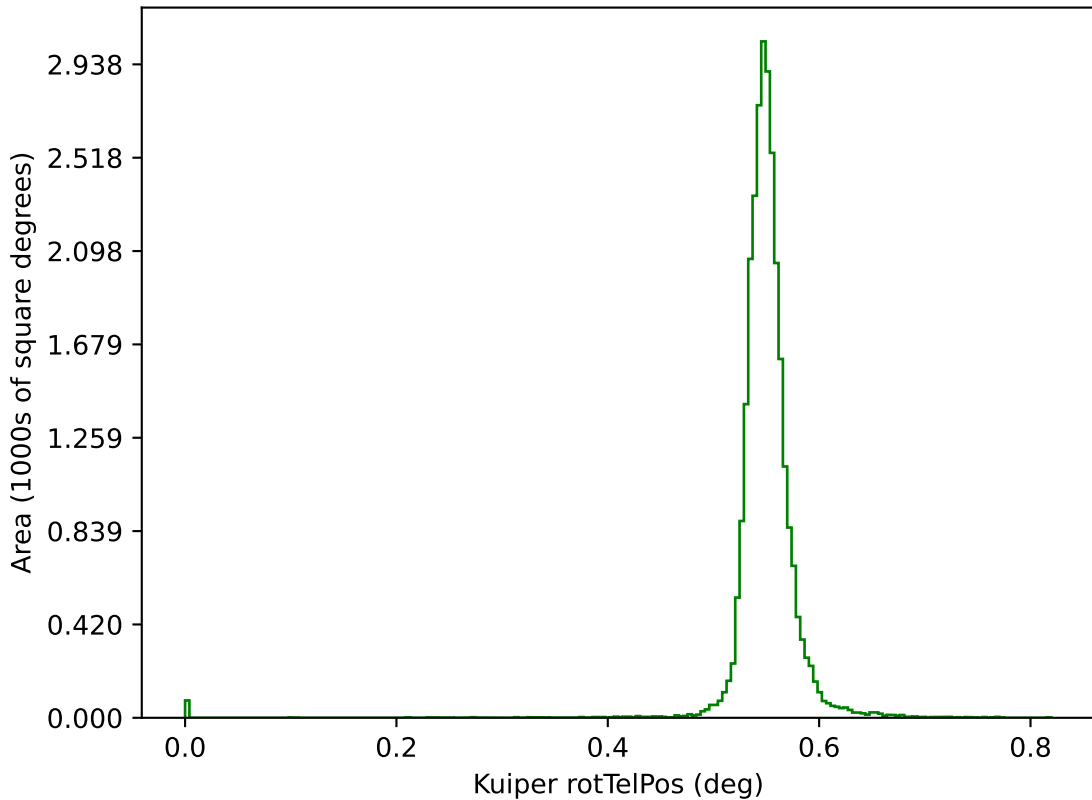
ddf_acor_sf20_ls40_lsr50_v3.4_10yrs g: Kuiper rotTelPos
