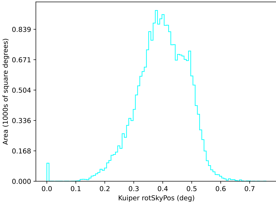
ddf_acor_sf20_lsf40_lsr50_v3.4_10yrs u: Kuiper rotSkyPos
