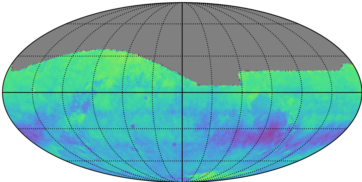
ddf_acor_sf20_lsf40_lsr50_v3.4_10yrs r: Kuiper rotSkyPos
