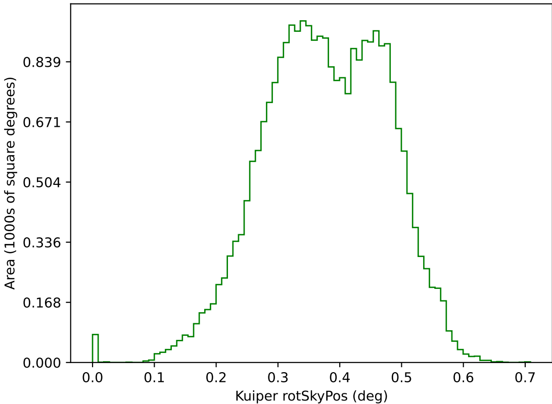
ddf_acor_sf20_lsf40_lsr50_v3.4_10yrs g: Kuiper rotSkyPos
