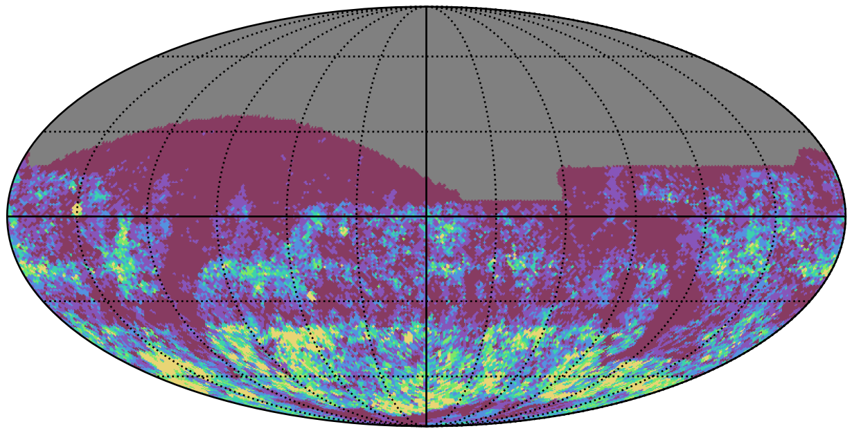
ddf_acor_sf20_lsf40_lsr50_v3.4_10yrs r band: Gaps_3hr
