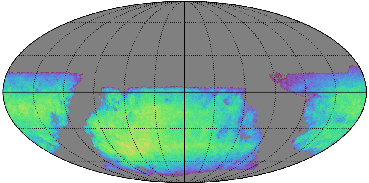
ddf_acor_sf20_lsf40_lsr50_v3.4_10yrs i band non-DD year 10: ExgalM5WithCuts
