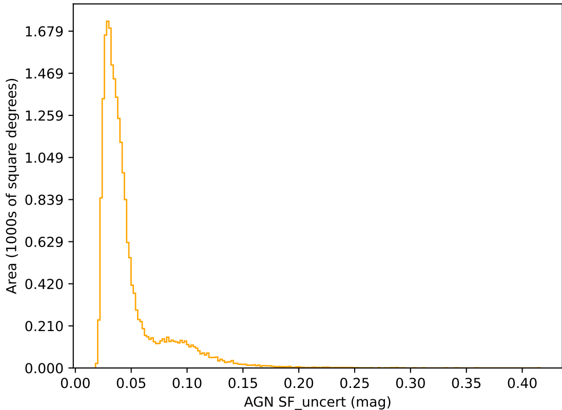
ddf_acor_sf20_lsf40_lsr50_v3.4_10yrs r band: AGN SF_uncert
