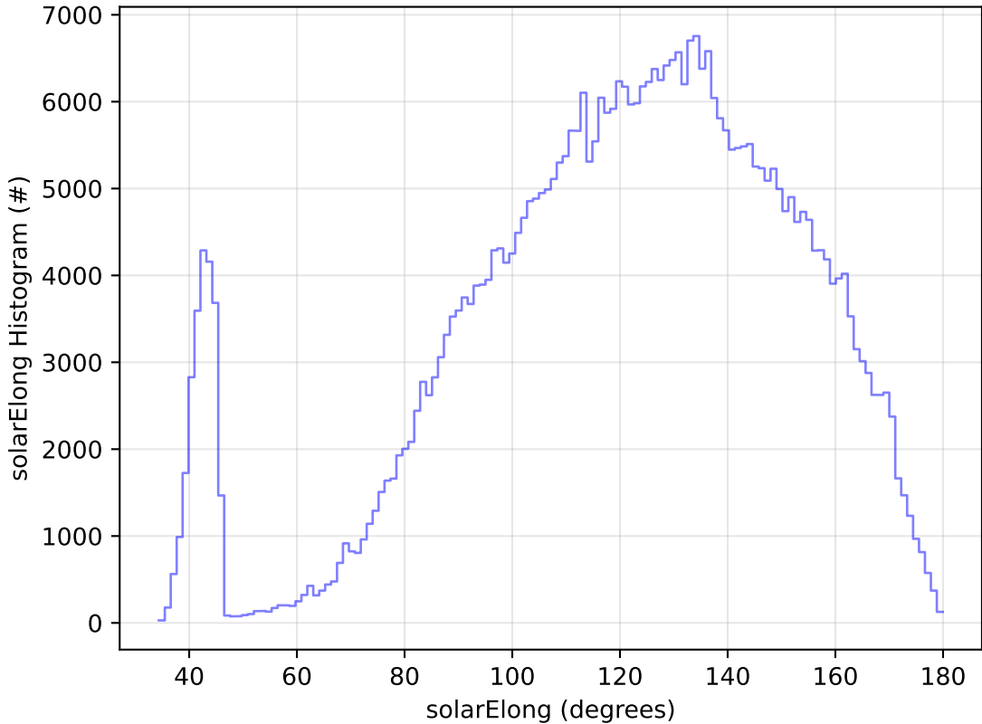
ddf_acor_sf20_lsf40_lsr50_v3.4_10yrs WFD z band: solarElong Histogram
