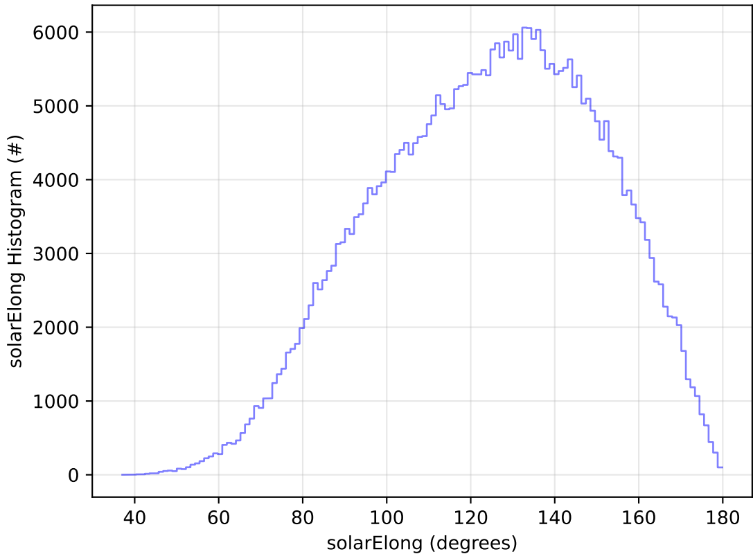
ddf_acor_sf20_lsf40_lsr50_v3.4_10yrs WFD y band: solarElong Histogram
