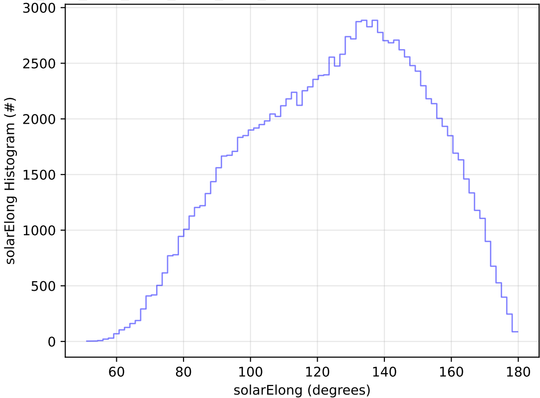
ddf_acor_sf20_lsf40_lsr50_v3.4_10yrs WFD u band: solarElong Histogram
