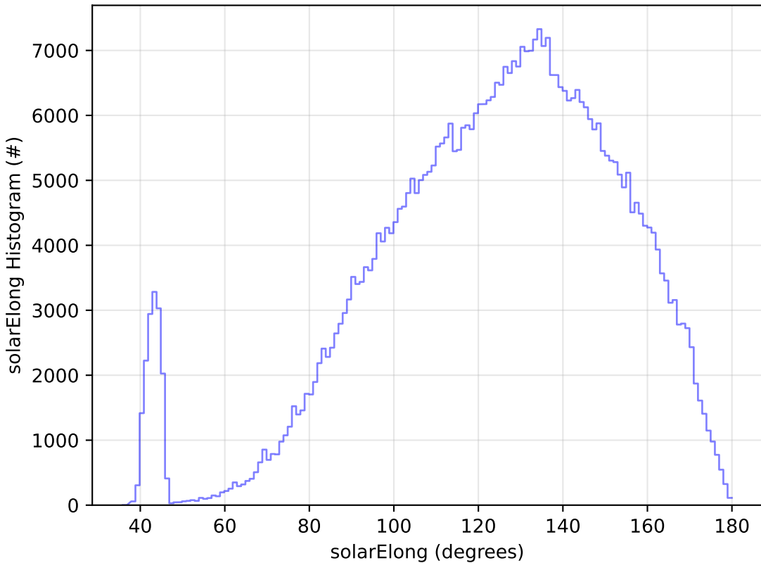
ddf_acor_sf20_lsf40_lsr50_v3.4_10yrs WFD r band: solarElong Histogram
