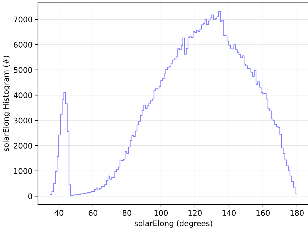
ddf_acor_sf20_lsf40_lsr50_v3.4_10yrs WFD i band: solarElong Histogram
