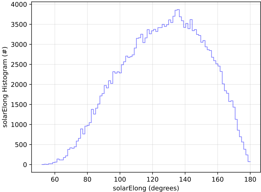
ddf_acor_sf20_lsf40_lsr50_v3.4_10yrs WFD g band: solarElong Histogram
