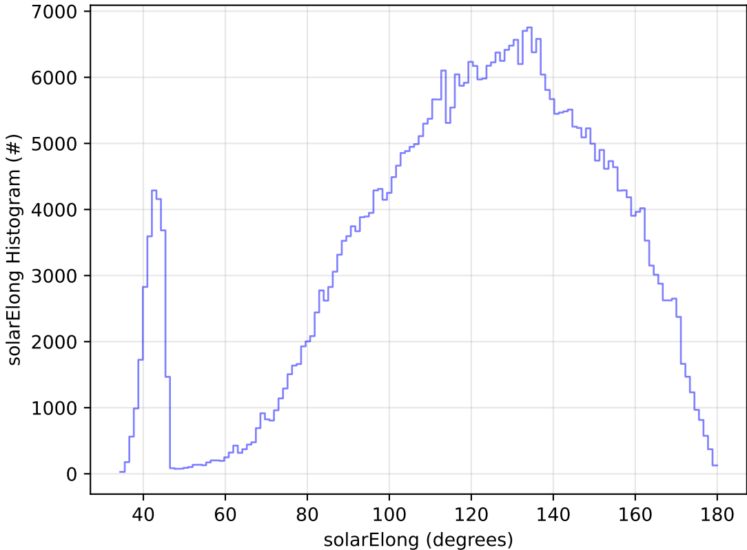
ddf_acor_sf20_lsf40_lsr50_v3.4_10yrs All sky z band: solarElong Histogram
