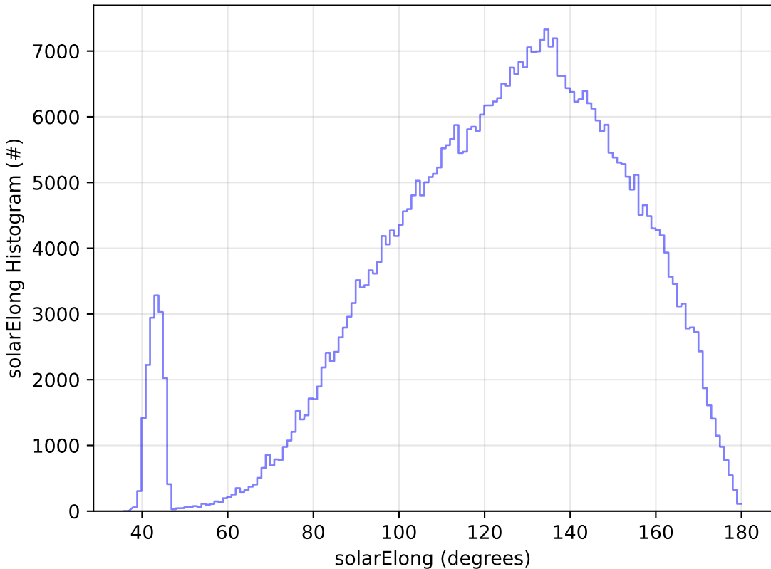
ddf_acor_sf20_lsf40_lsr50_v3.4_10yrs All sky r band: solarElong Histogram
