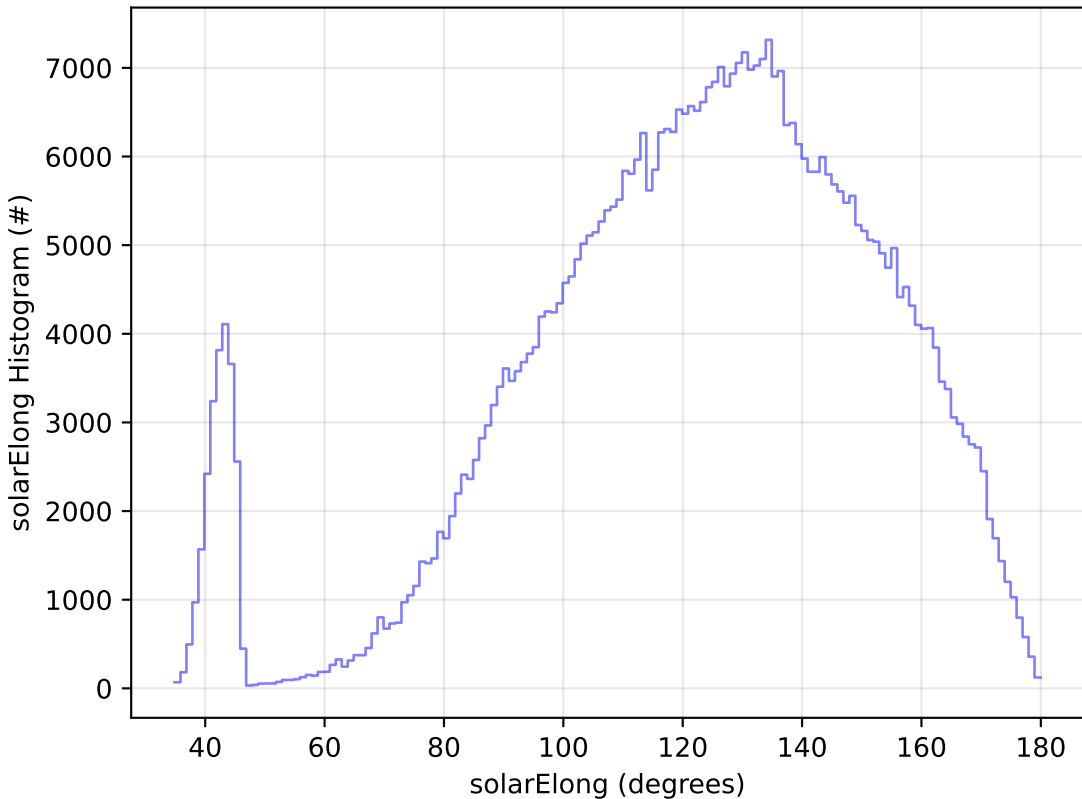
ddf_acor_sf20_lsf40_lsr50_v3.4_10yrs All sky i band: solarElong Histogram
