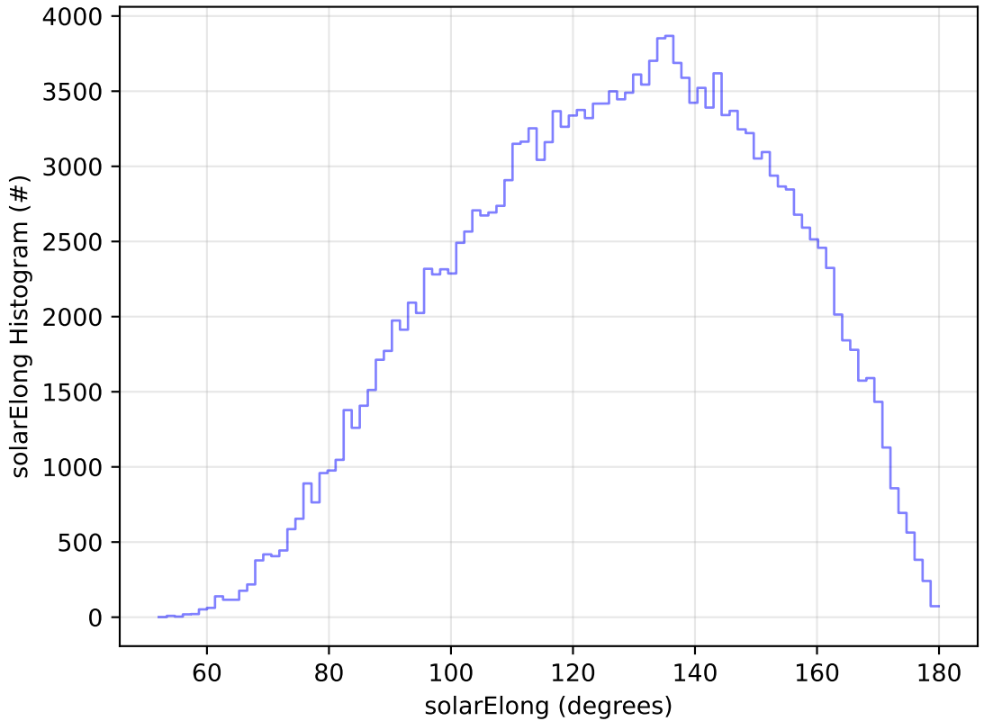
ddf_acor_sf20_lsf40_lsr50_v3.4_10yrs All sky g band: solarElong Histogram
