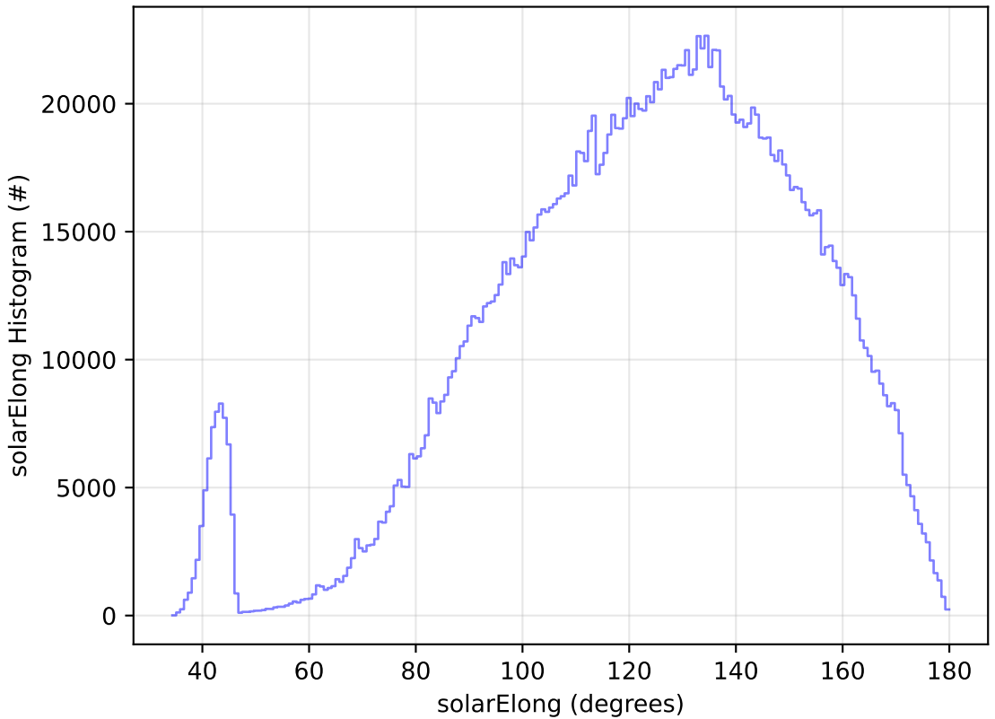
ddf_acor_sf20_lsf40_lsr50_v3.4_10yrs All sky all bands: solarElong Histogram
