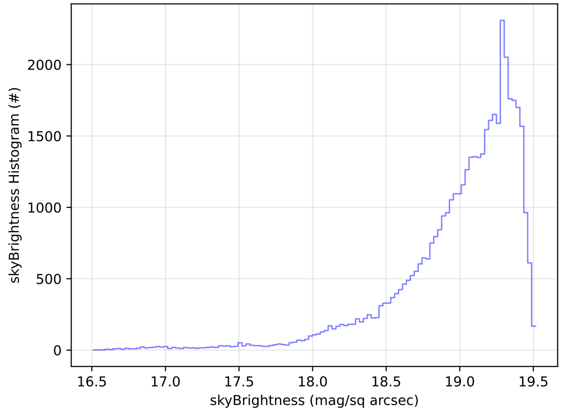
ddf_acor_sf20_lsf40_lsr50_v3.4_10yrs Yr 1 z band: skyBrightness Histogram
