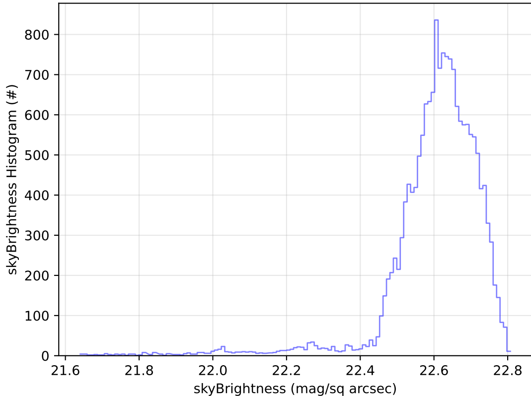
ddf_acor_sf20_lsf40_lsr50_v3.4_10yrs Yr 1 u band: skyBrightness Histogram
