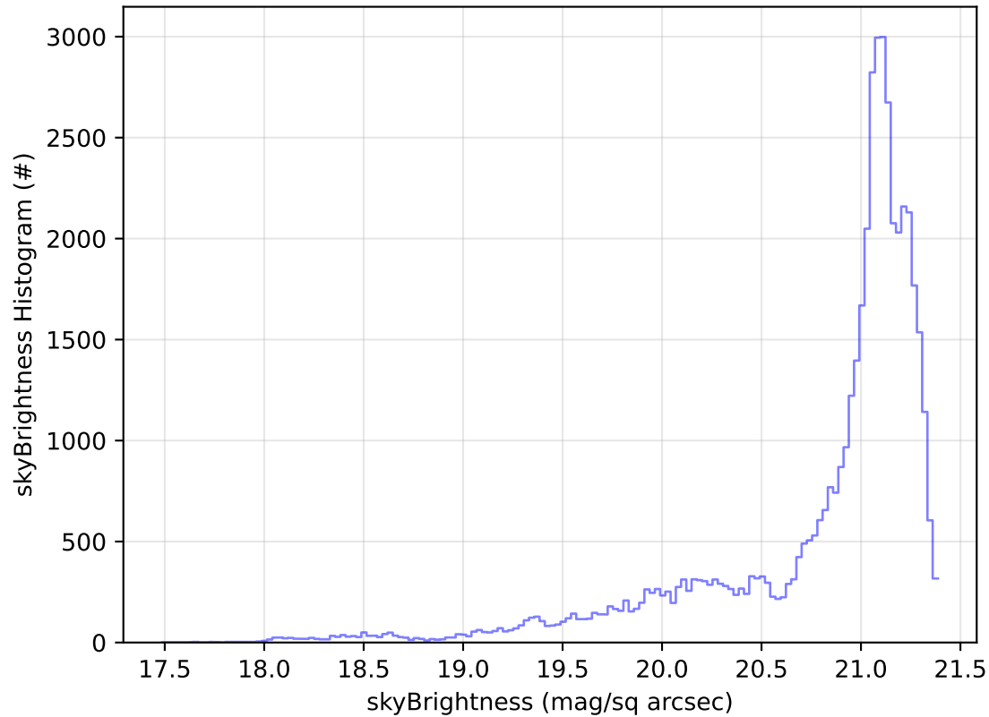
ddf_acor_sf20_lsf40_lsr50_v3.4_10yrs Yr 1 r band: skyBrightness Histogram
