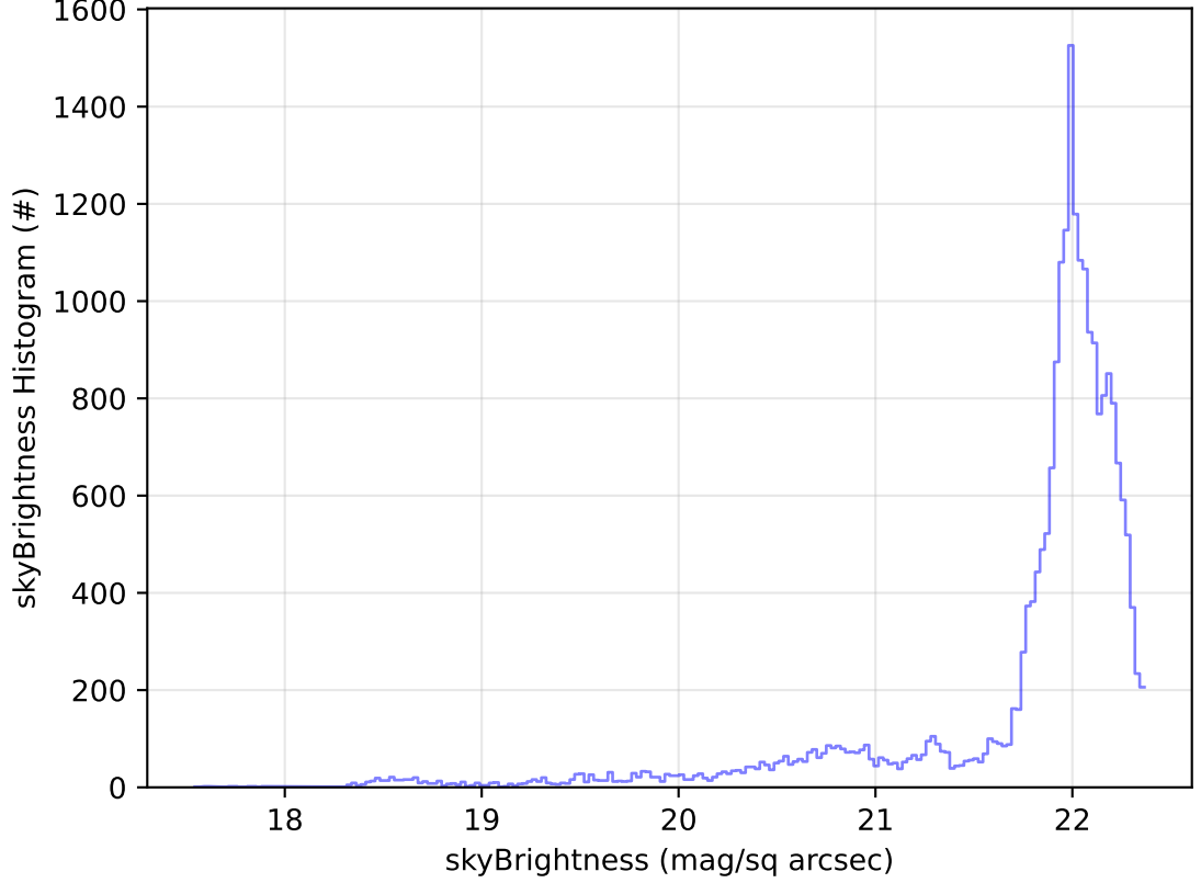
ddf_acor_sf20_lsf40_lsr50_v3.4_10yrs Yr 1 g band: skyBrightness Histogram
