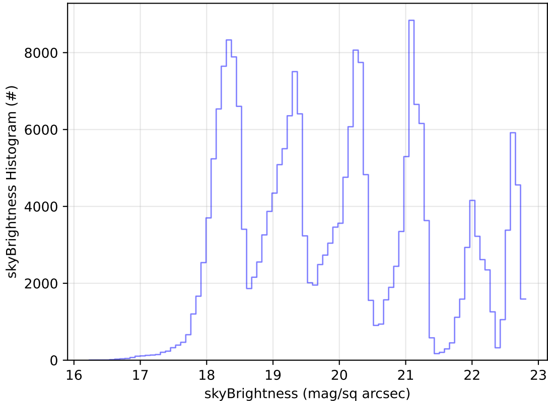
ddf_acor_sf20_lsf40_lsr50_v3.4_10yrs Yr 1 all bands: skyBrightness Histogram
