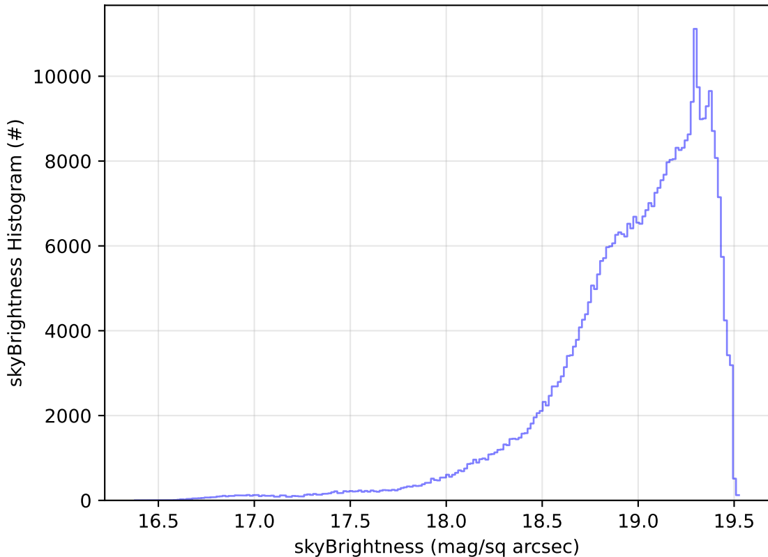
ddf_acor_sf20_lsf40_lsr50_v3.4_10yrs WFD z band: skyBrightness Histogram
