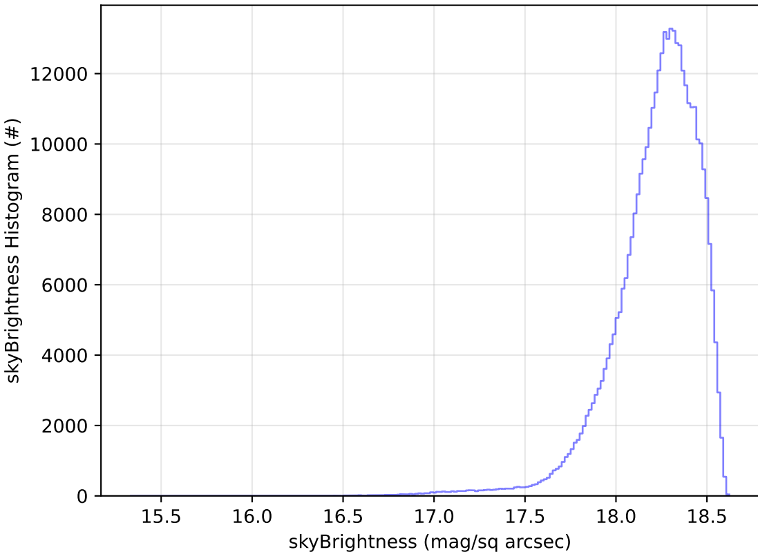
ddf_acor_sf20_lsf40_lsr50_v3.4_10yrs WFD y band: skyBrightness Histogram
