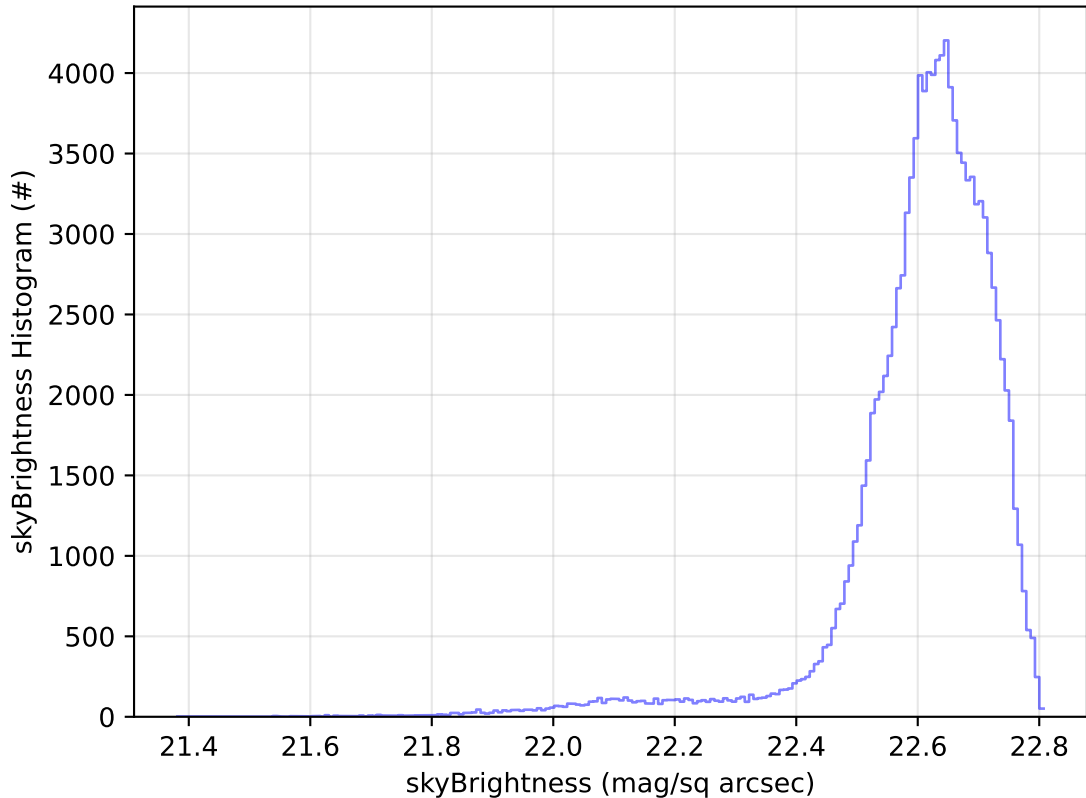
ddf_acor_sf20_lsf40_lsr50_v3.4_10yrs WFD u band: skyBrightness Histogram
