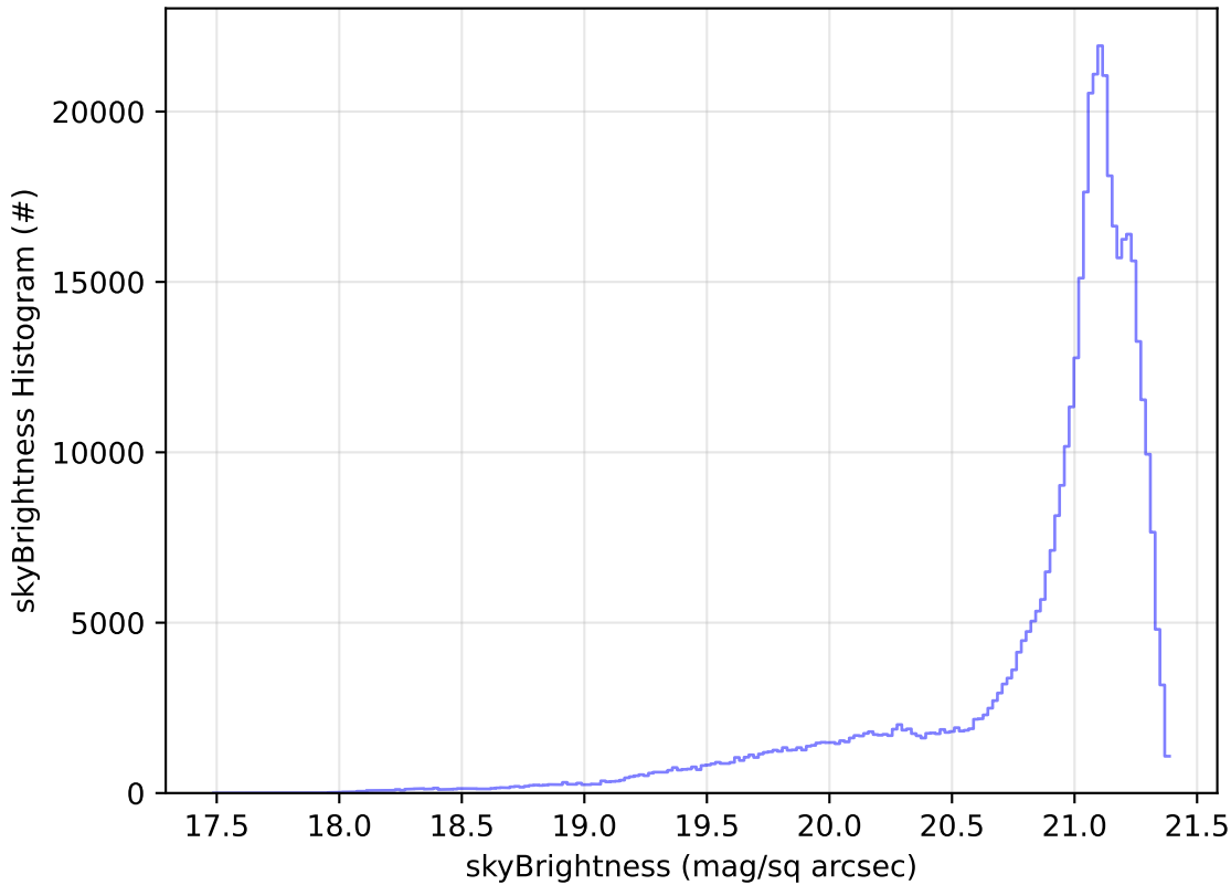
ddf_acor_sf20_lsf40_lsr50_v3.4_10yrs WFD r band: skyBrightness Histogram
