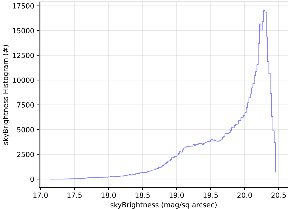
ddf_acor_sf20_lsf40_lsr50_v3.4_10yrs WFD i band: skyBrightness Histogram
