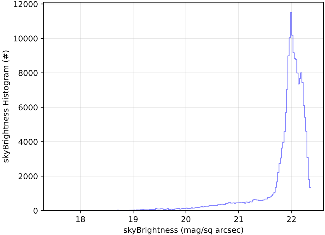
ddf_acor_sf20_lsf40_lsr50_v3.4_10yrs WFD g band: skyBrightness Histogram
