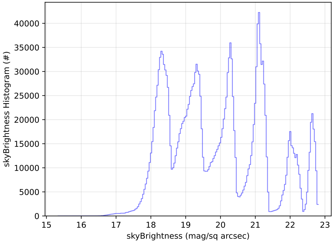
ddf_acor_sf20_lsf40_lsr50_v3.4_10yrs WFD all bands: skyBrightness Histogram
