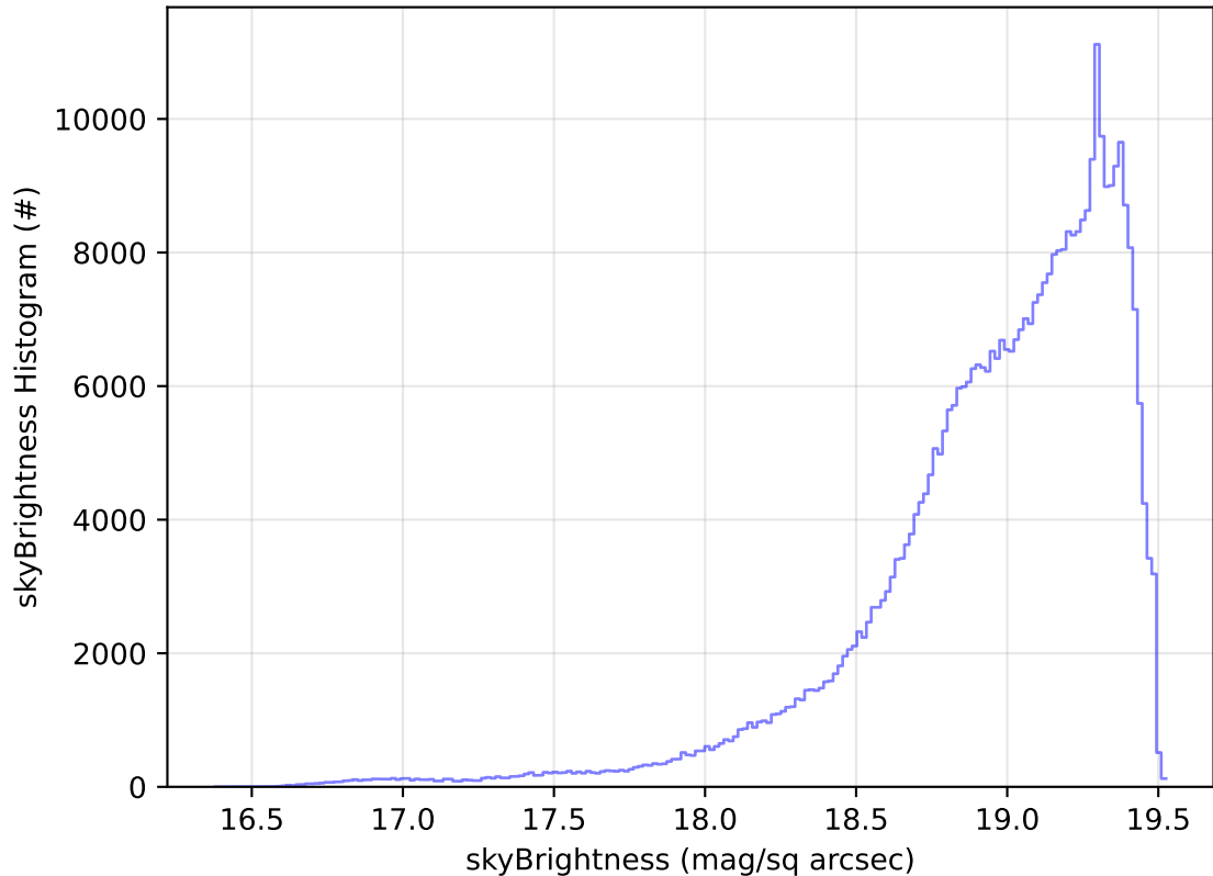
ddf_acor_sf20_lsf40_lsr50_v3.4_10yrs All sky z band: skyBrightness Histogram
