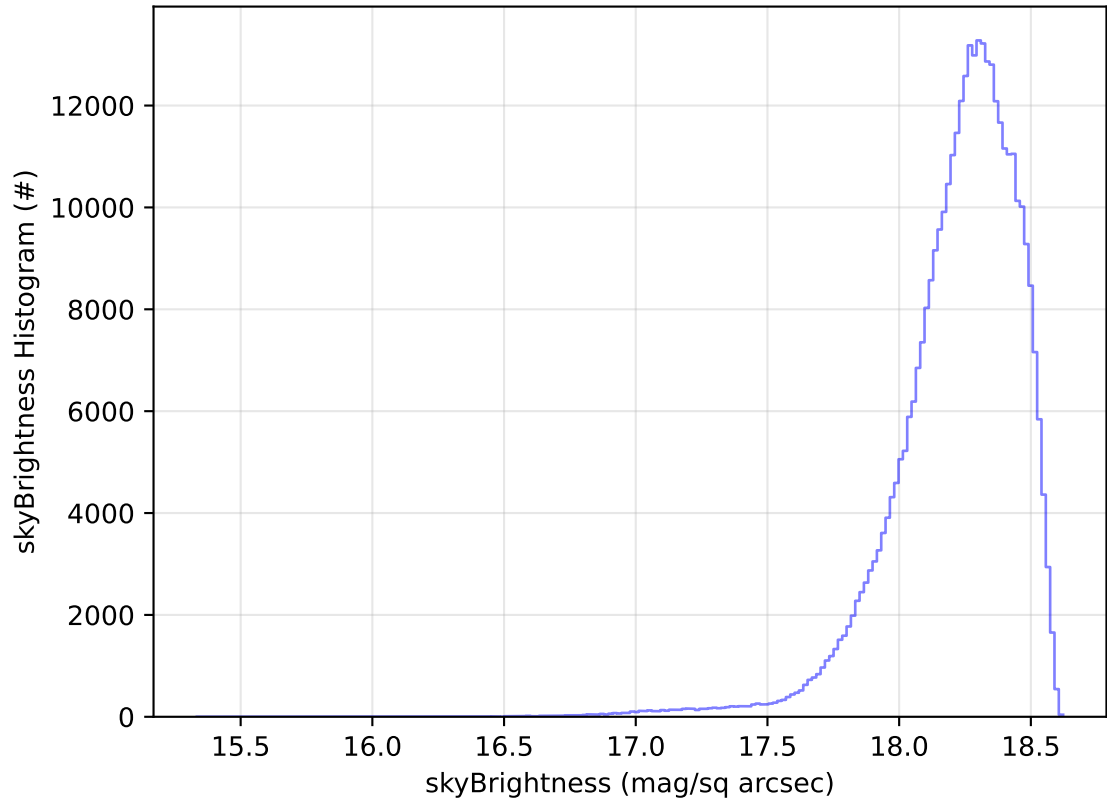
ddf_acor_sf20_lsf40_lsr50_v3.4_10yrs All sky y band: skyBrightness Histogram
