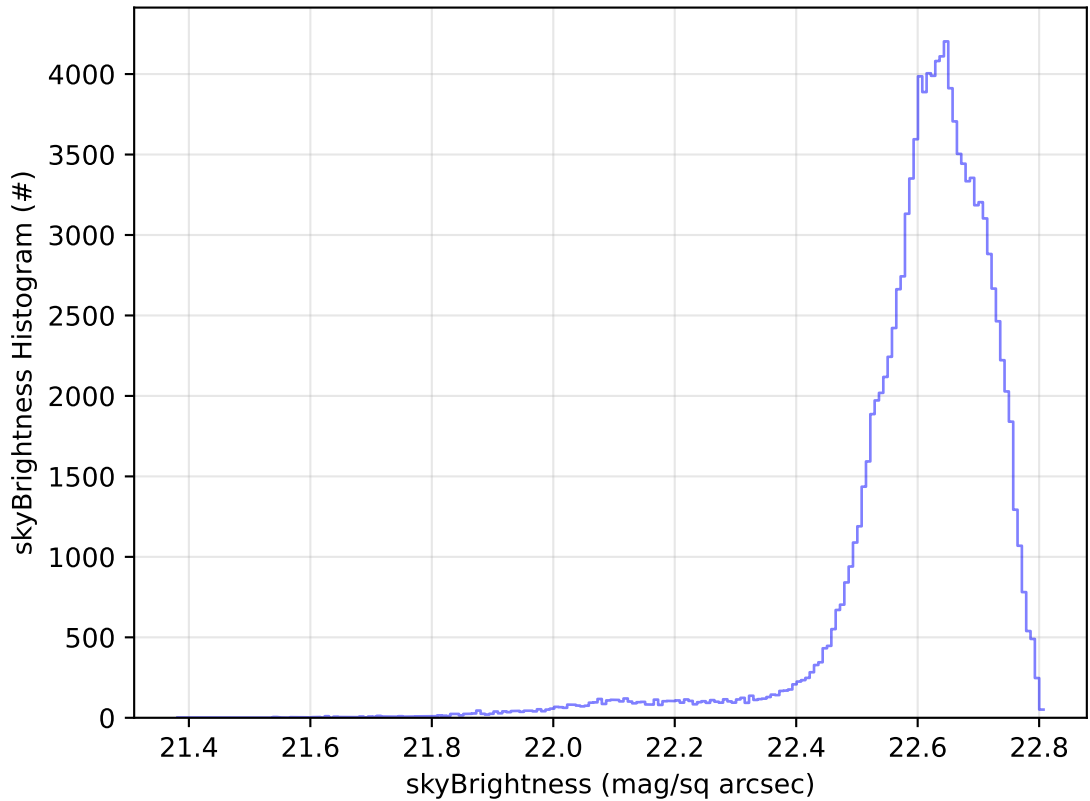
ddf_acor_sf20_lsf40_lsr50_v3.4_10yrs All sky u band: skyBrightness Histogram
