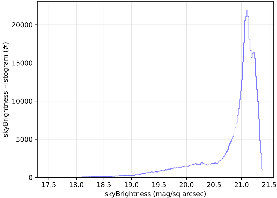
ddf_acor_sf20_lsf40_lsr50_v3.4_10yrs All sky r band: skyBrightness Histogram
