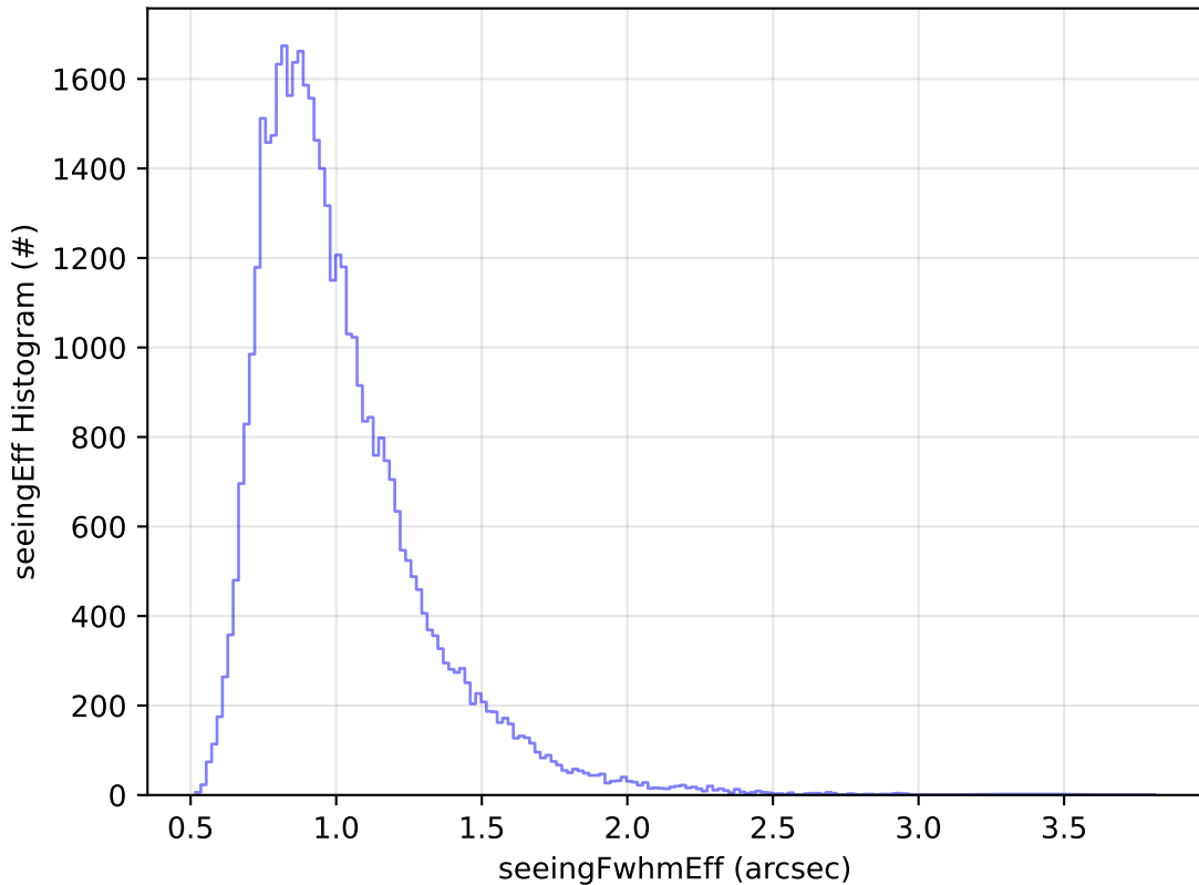
ddf_acor_sf20_lsf40_lsr50_v3.4_10yrs Yr 1 z band: seeingEff Histogram
