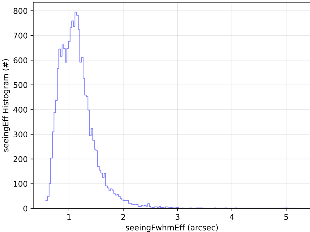
ddf_acor_sf20_lsf40_lsr50_v3.4_10yrs Yr 1 u band: seeingEff Histogram
